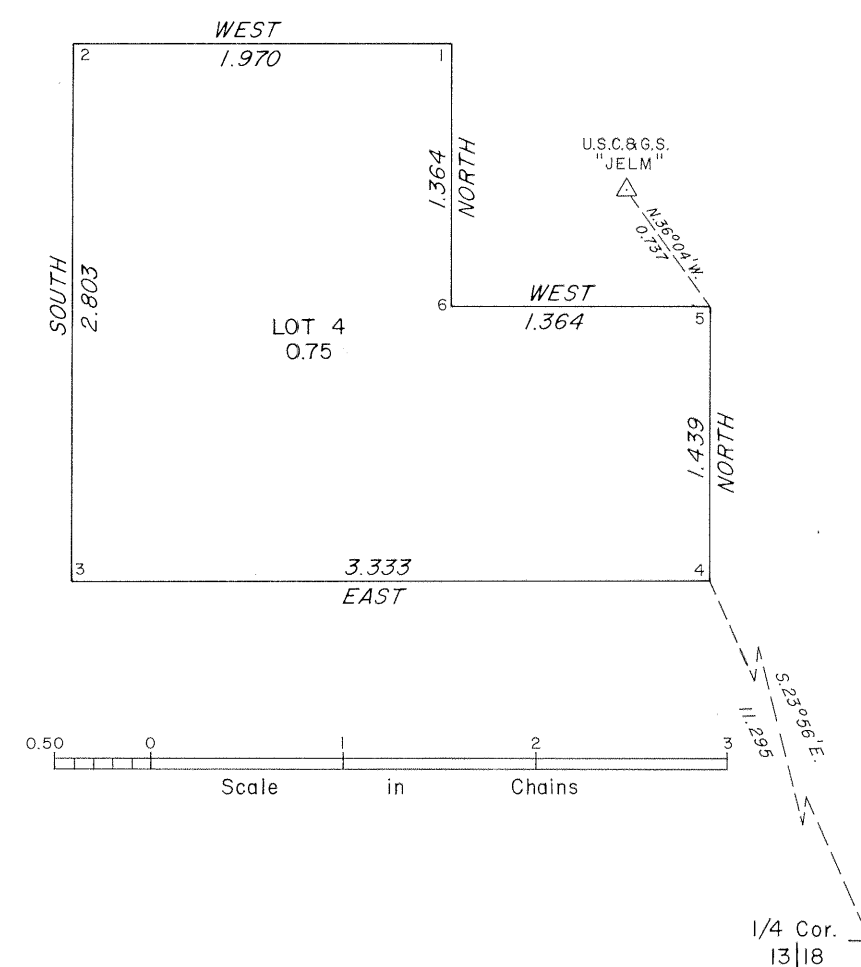
ENLARGED DIAGRAM
