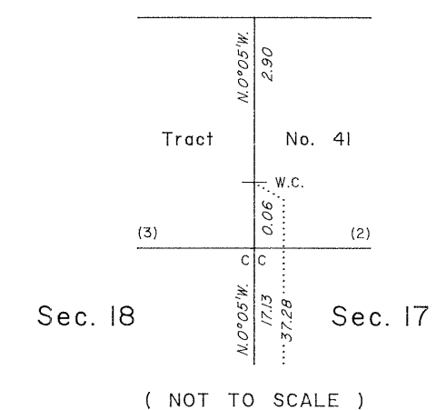
ENLARGED DIAGRAM
