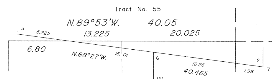
ENLARGED DIAGRAM
