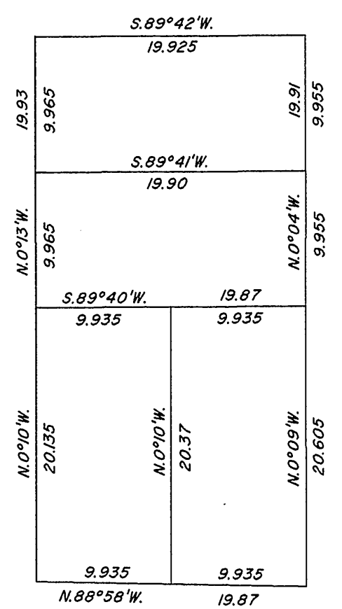
DETAIL "A" SW1/4NW1/4 and NW1/4SW1/4 Sec. 1
