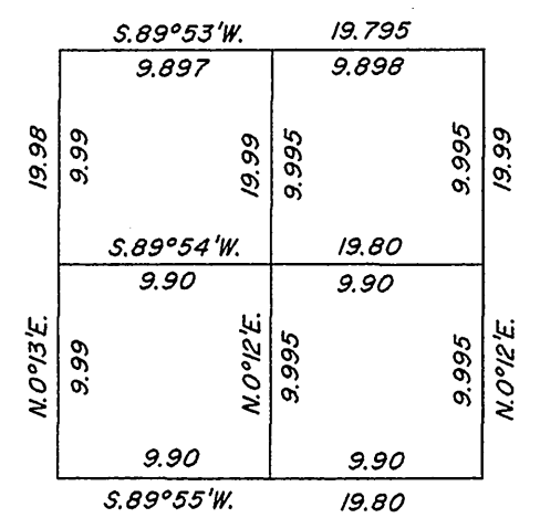
DETAIL "B" NE1/4SE1/4 Sec. 8
