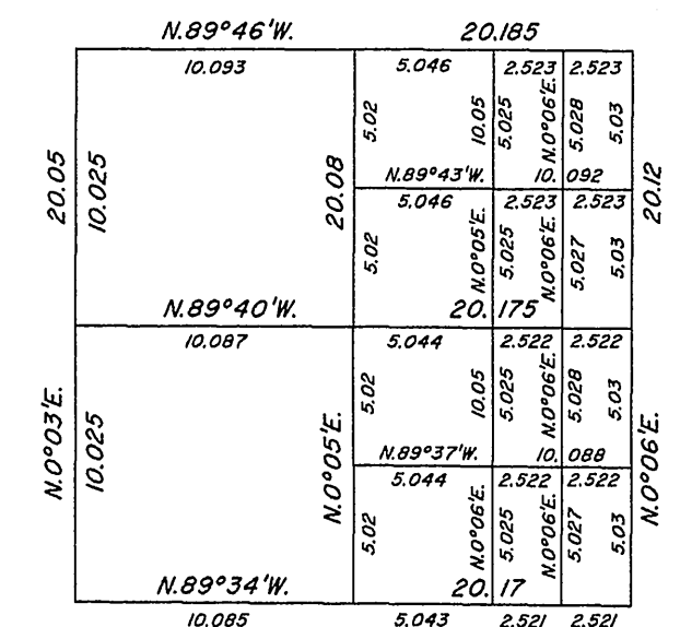
DETAIL "C" NW1/4SE1/4 Sec. 13
