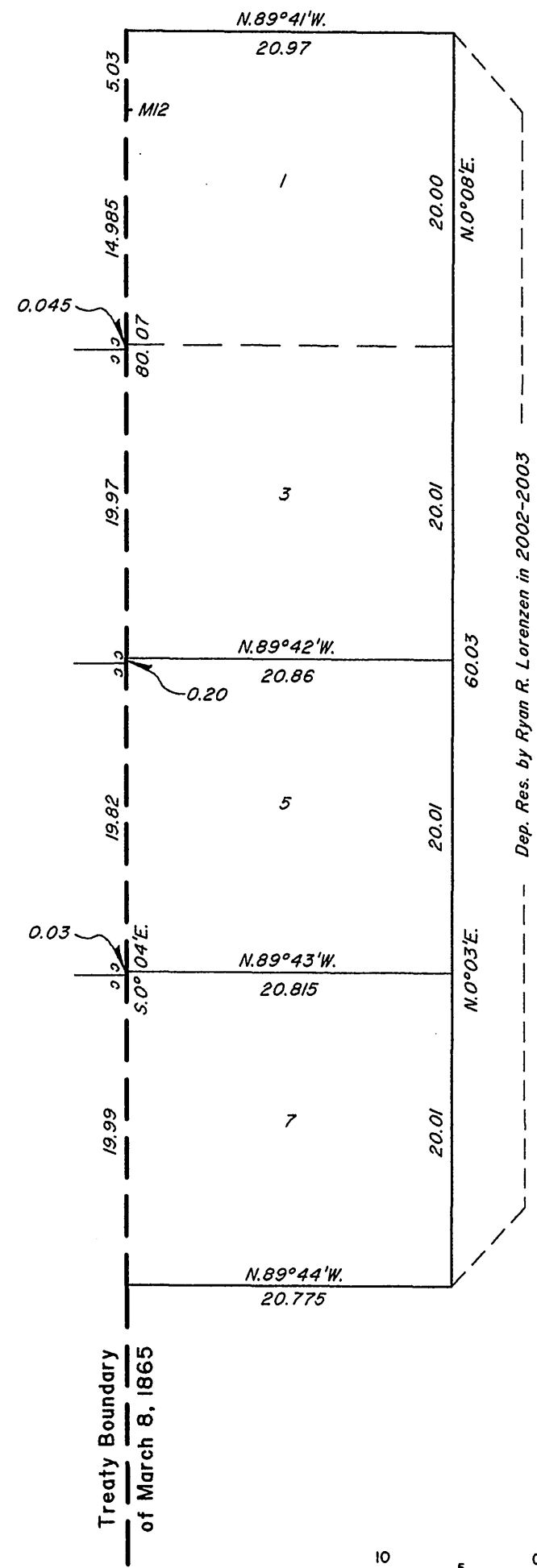
DETAIL "D" Sec. 25
