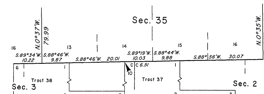
ENLARGED DIAGRAM "B"
