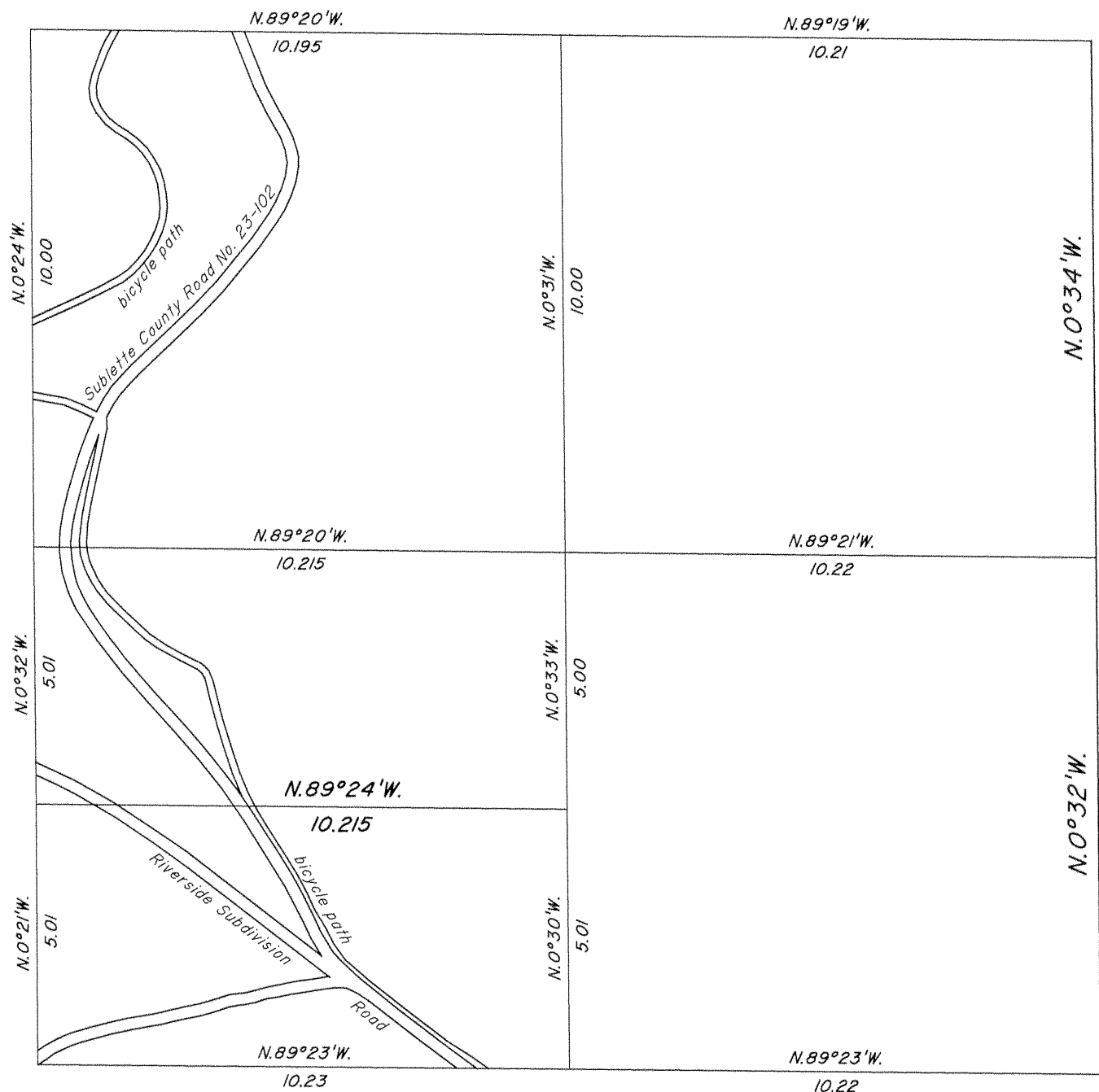
ENLARGED DIAGRAM
